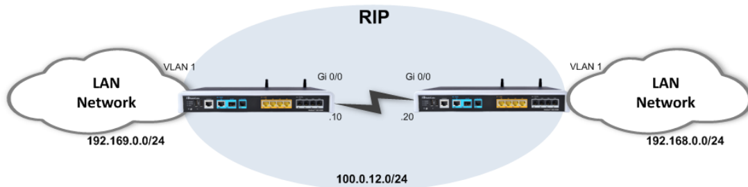
Figure 11-1: RIP Routing
