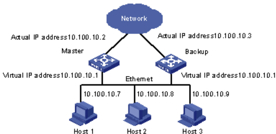
Figure 4-1: VRRP Example
