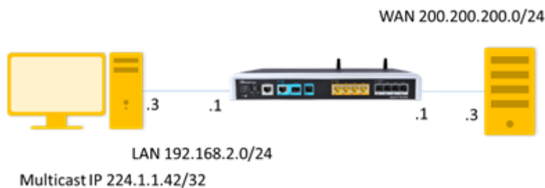
Figure 22-1 Multicast Example – IGMP Proxy
