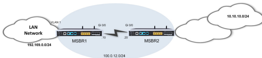
Figure 8-1: Static Routing
