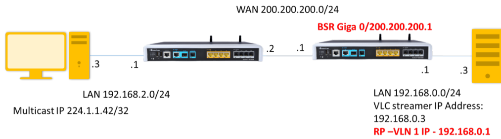
Figure 21-9: Setup Description
