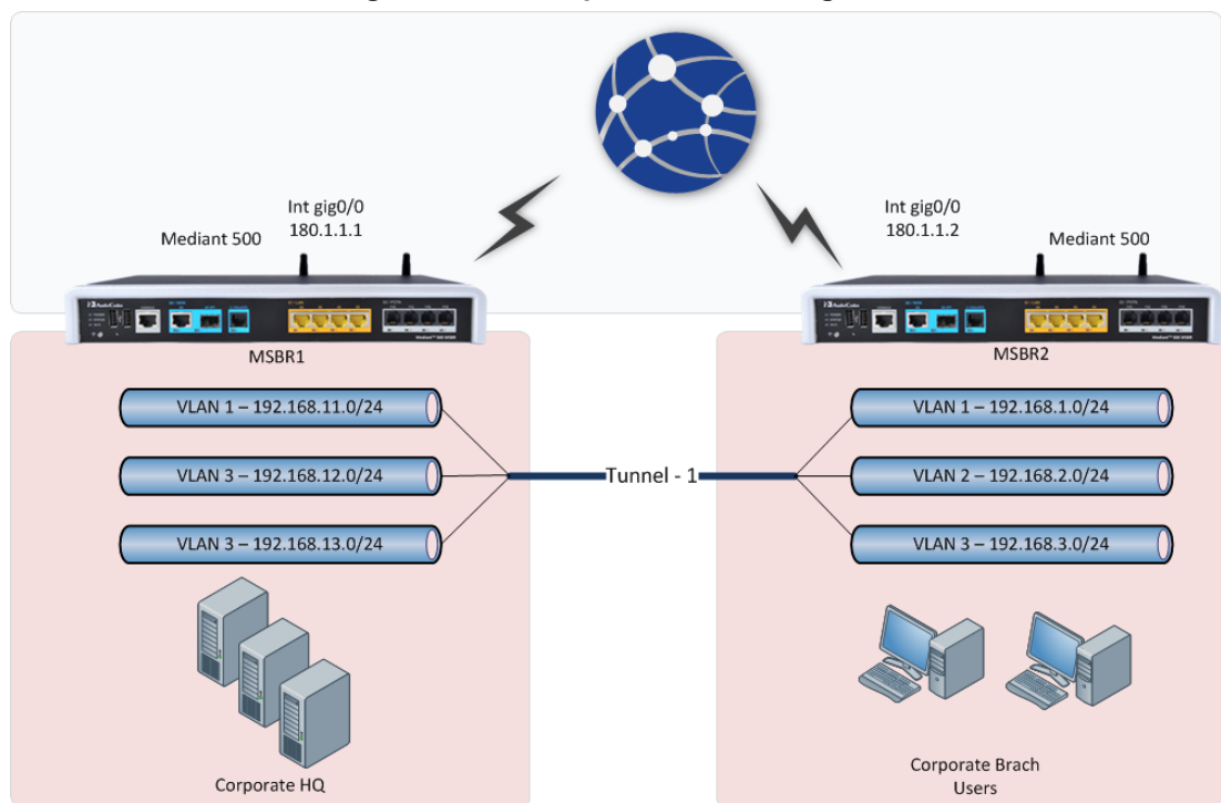
Figure 15-1: Multiple Subnets using GRE
