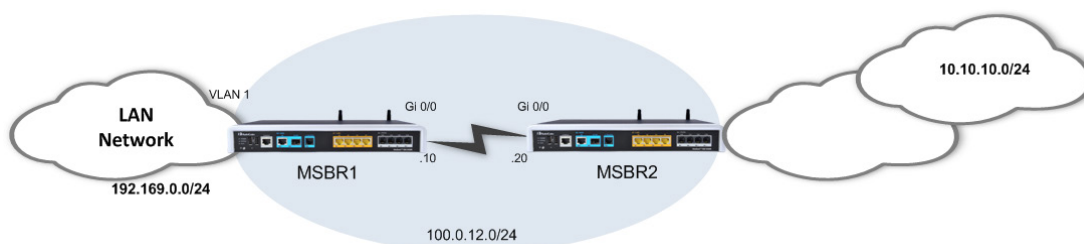
Figure 10-2: Changing Static Route Metric
