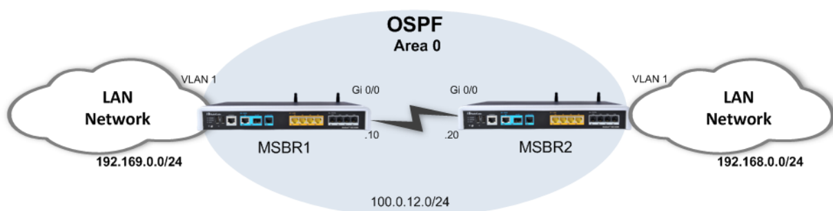
Figure 11-2: OSPF Routing
