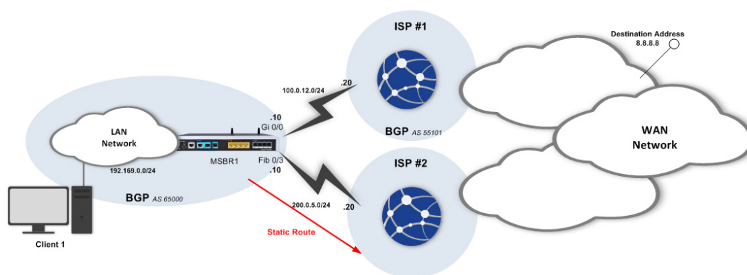
Figure 11-5: Multi-Wan with Floating Static Route
