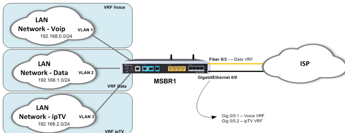
Figure 14-2: Routing Services on Different VRFs
