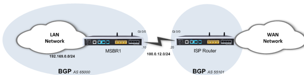
Figure 11-3: Basic BGP Routing
