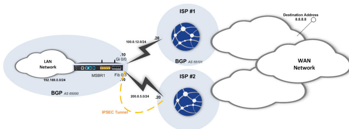
Figure 11-6: Multi WAN with BGP and IPsec
