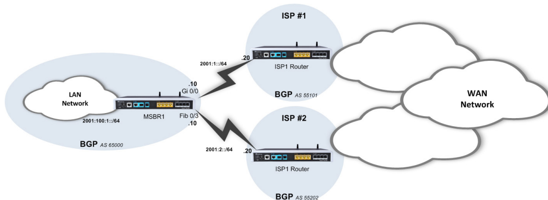
Figure 20-5: BGP IPv6 Example 2
