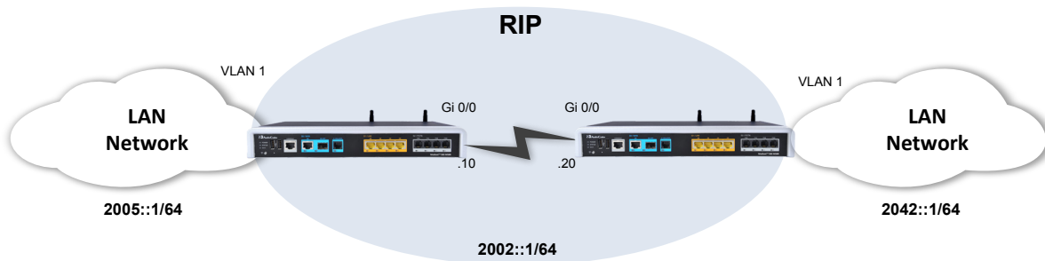
Figure 20-2: RIPng Routing
