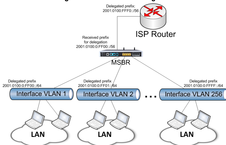
Figure 20-6: IPv6 Prefix Delegation
