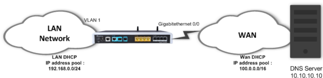
Figure 6-2: Static DNS
