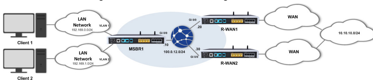
Figure 8-2: Multi WAN with Floating Static Route
