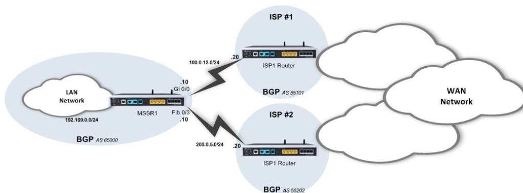
Figure 11-4: BGP Multi-WAN
