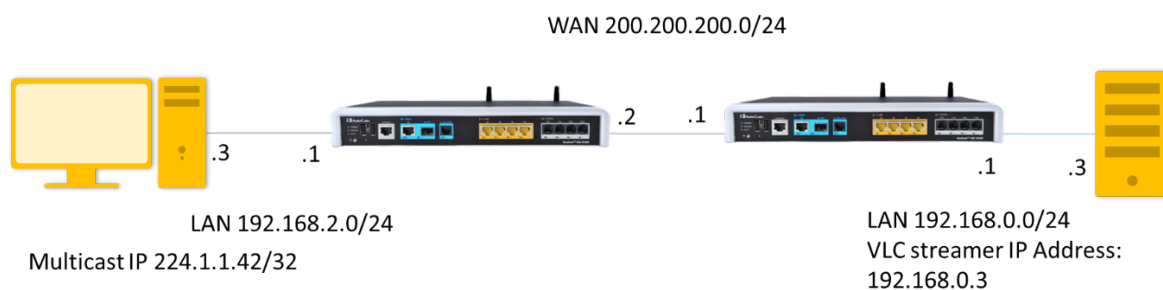
Figure 21-1: Multicast Example - Static RP
