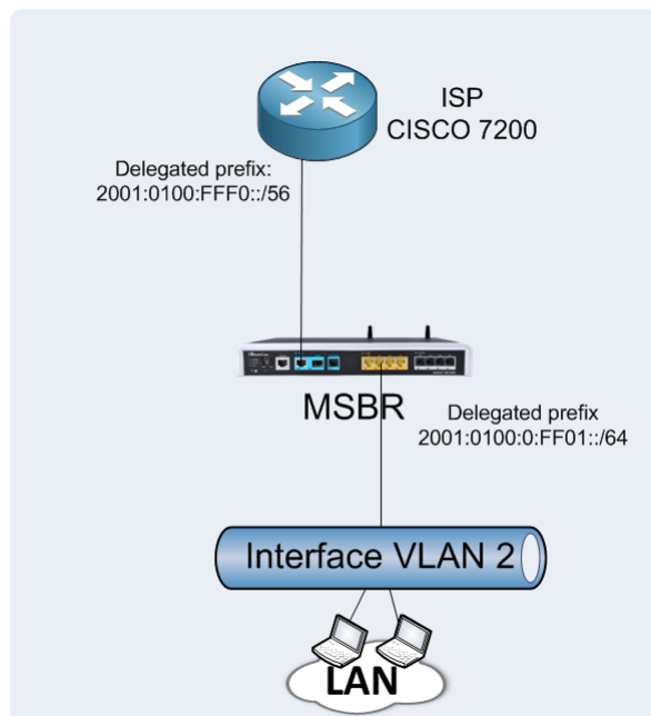
Figure 20-7: DHCPv6 Prefix Delegation Example
